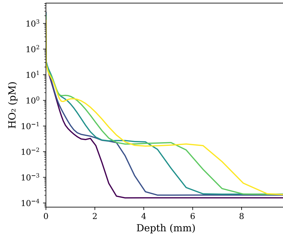
(f) \text{HO}_2
